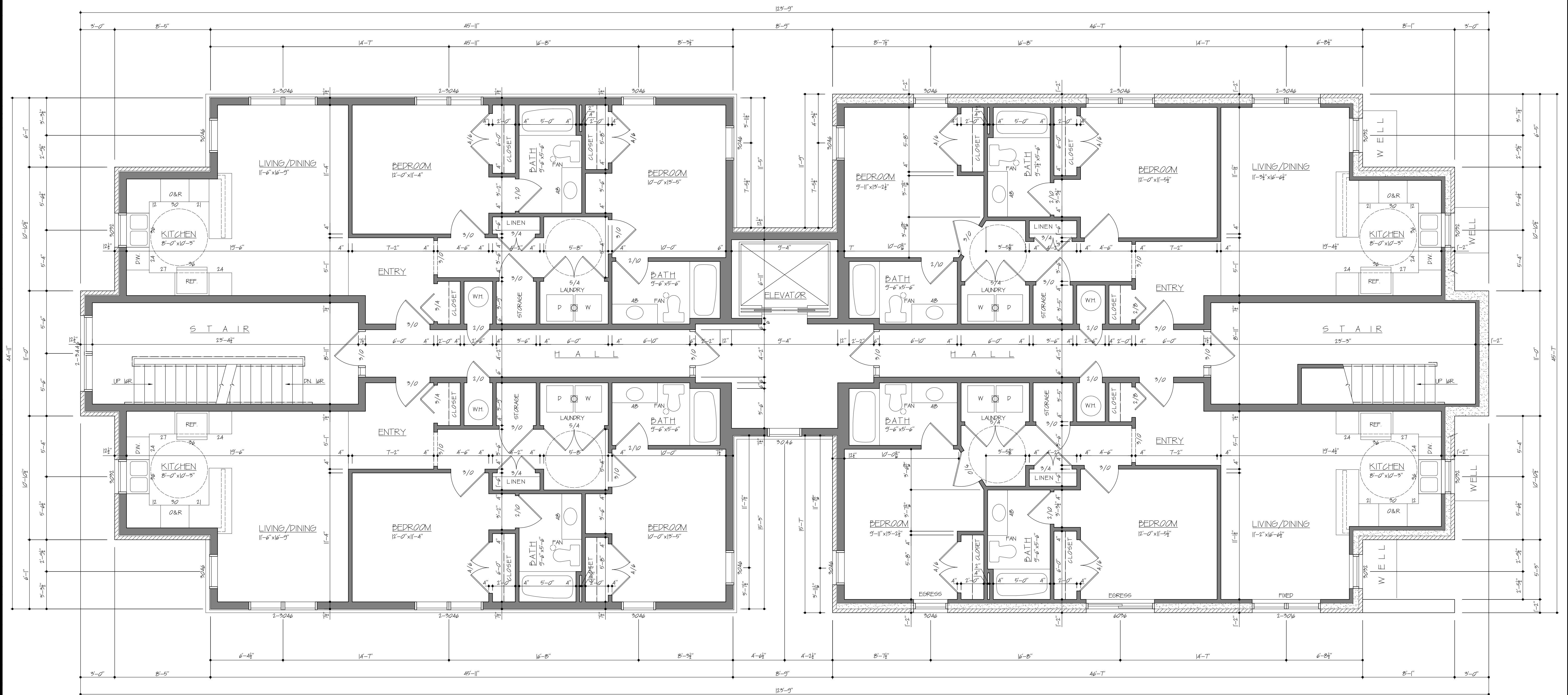
LEVEL TWO PLAN SCALE 1/4" = 1'-0"
